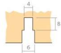
Double morticed for small gaps
