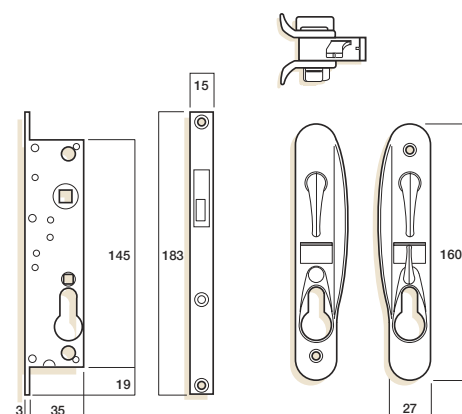
Cylinder locking
