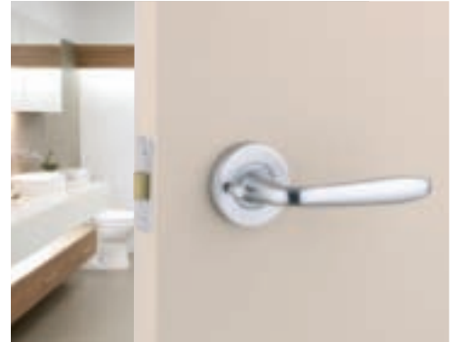
Inside view of privacy leverset with inside locking button. This set also features auto release (by turning the inside lever) and emergency access from the outside.
