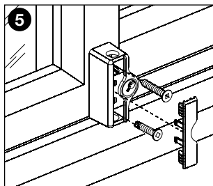
Attach lock to frame
