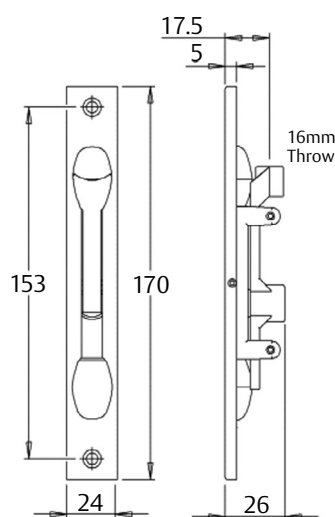
Surface Mounted
